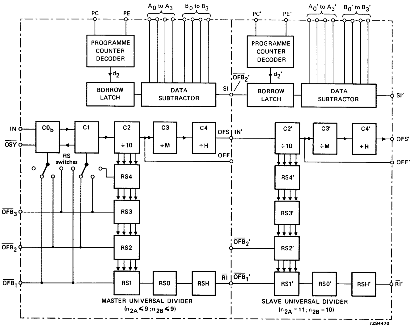
Fig.8 Block diagram showing cascading of U.Ds.
