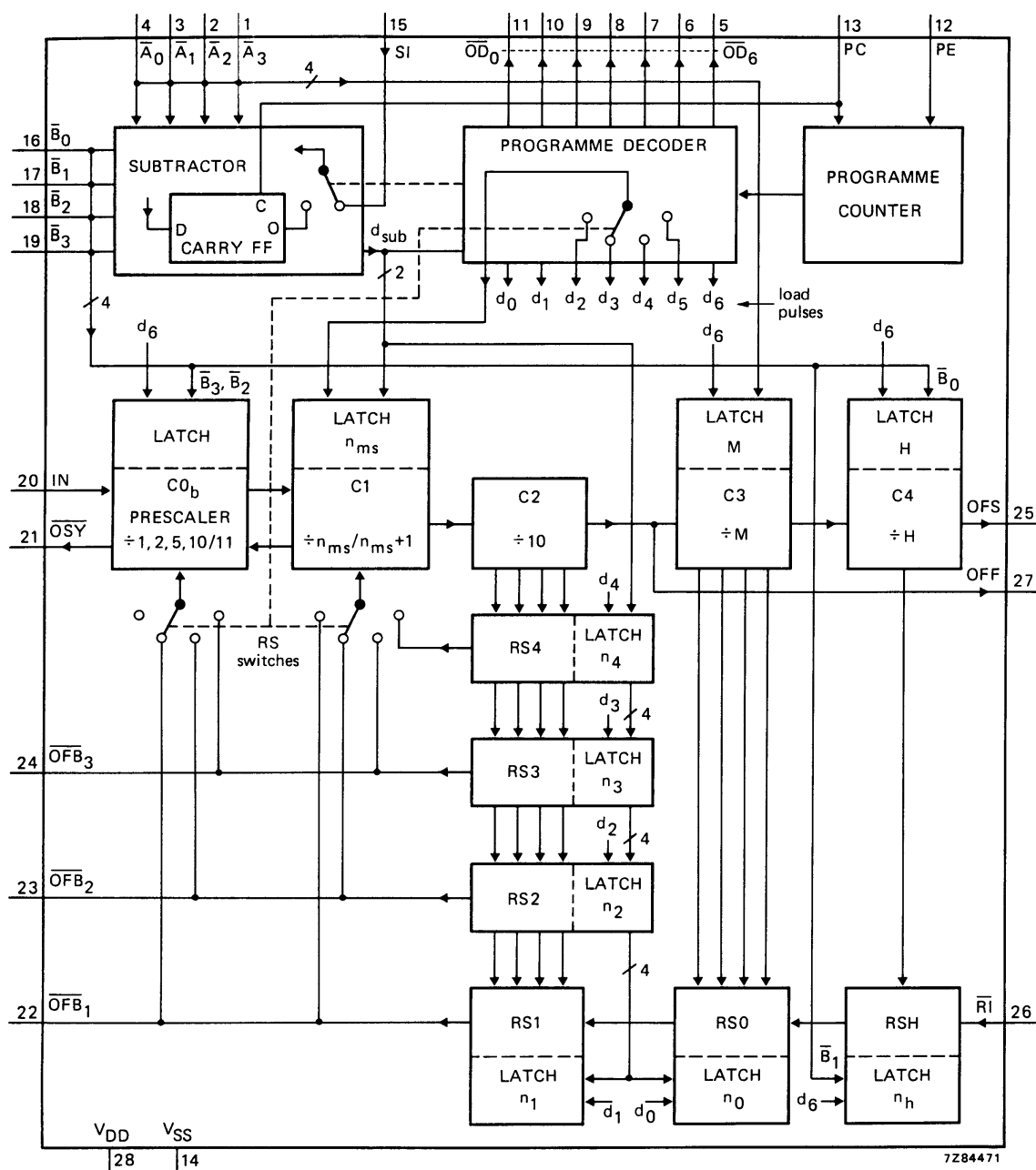
Fig.2 Block diagram.
