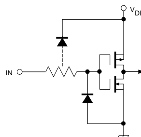
TYPICAL INPUT CIRCUIT
