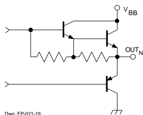
TYPICAL OUTPUT DRIVER
